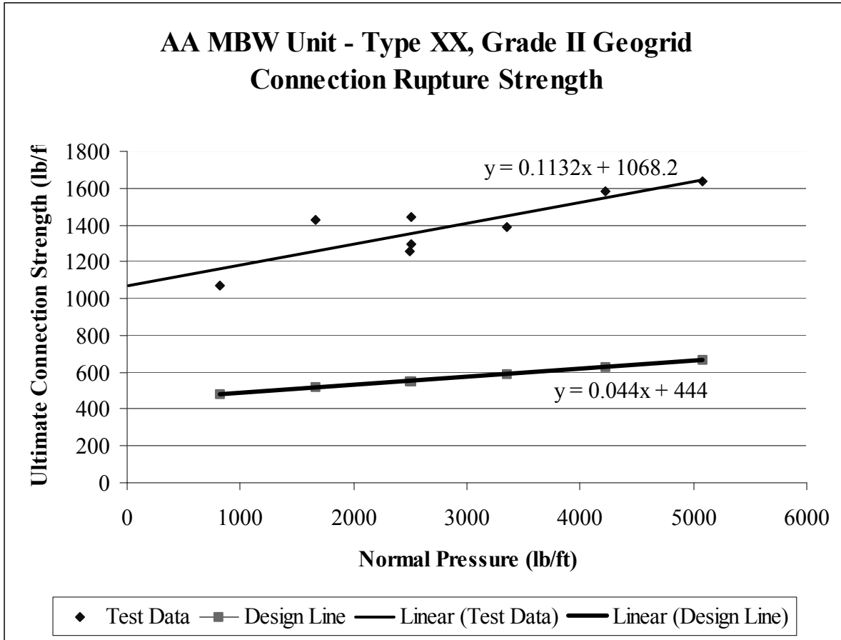
Figure B-5. Laboratory test data and the nominal long-term connection strength lines for AA MBW unit and Type XX, Grade II geogrid.
