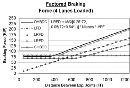
Figure C3.6.4-1 (continued)—Comparison of Braking Force Models
