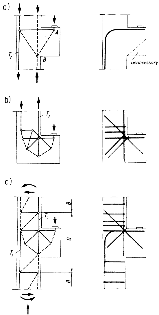
Figure C5.13.2.4.1-1—Different Support Conditions Leading to Different Strut-and-Tie Models and Different Reinforcement Arrangements of Corbels and Beam Ledges (Schlaich et al., 1987)
