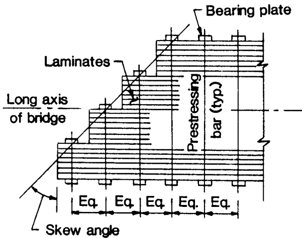
Figure 9.9.5.6.1-2—Staggered Layout of Prestressing Bars in End Zone of Skewed Decks—Illustrative Only
