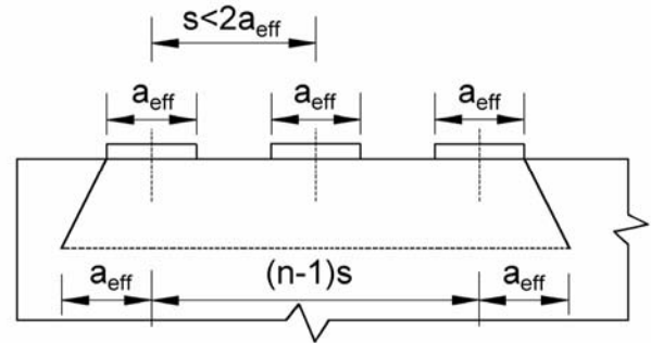
Figure C5.10.9.6.2-2—Closely Spaced Multiple Anchorages
