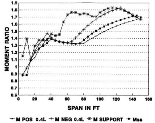
Figure C3.6.1.2.1-1—Moment Ratios: Exclusion Vehicles to HS20 (truck or lane) or Two 24.0-kip Axles at 4.0 ft
