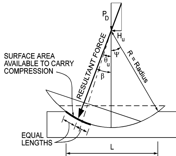
Figure C14.7.3.3-1—Bearing Geometry
