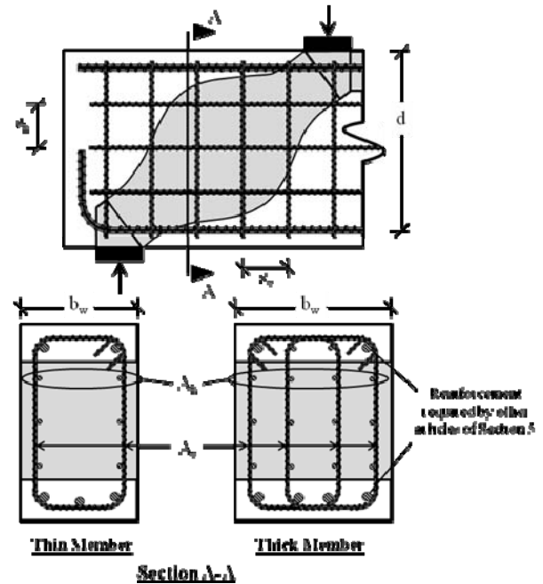
Figure C5.6.3.6-1—Distribution of Crack Control Reinforcement in Compression Strut
