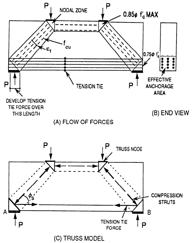
Figure C5.6.3.2-1—Strut-and-Tie Model for a Deep Beam
