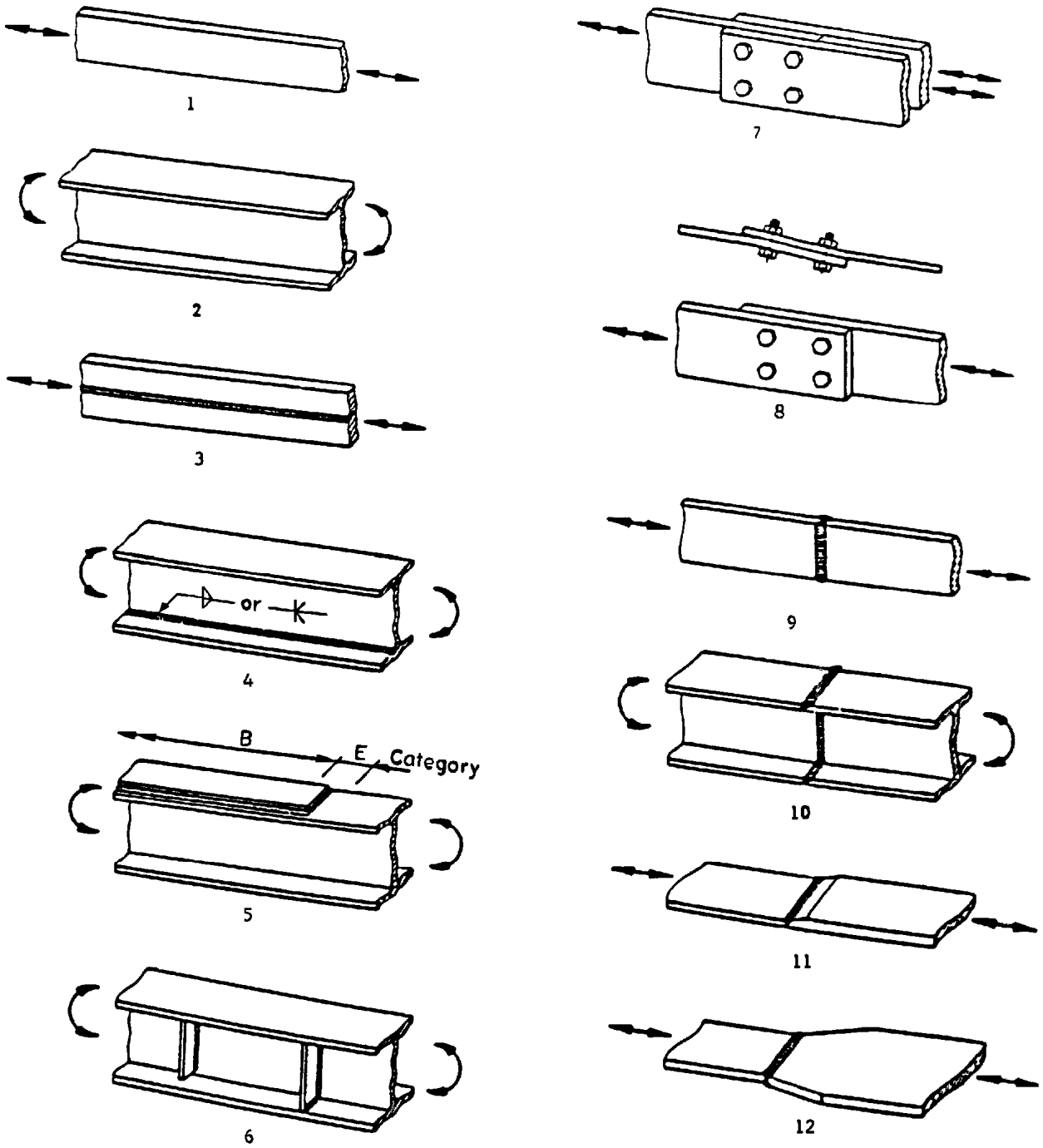
Figure 7.6.1.2.3-1—Illustrative Examples
