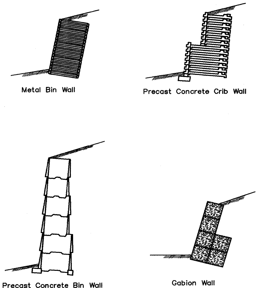
Figure C11.11.1-1—Typical Prefabricated Modular Gravity Walls
