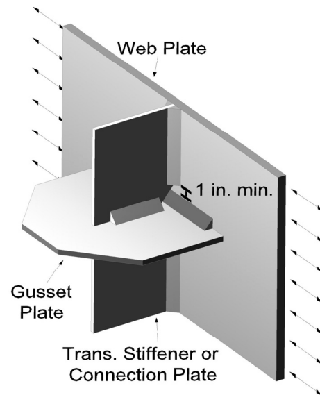
Figure C6.6.1.3.2-1—Typical Discontinuous Transverse Stiffener Detail at a Lateral Connection Plate
