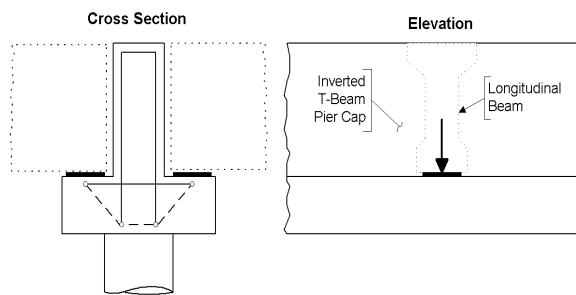
Figure C5.8.3.2-3—Inverted T-Beam Pier Cap
