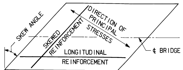
Figure C9.7.1.3-1—Reinforcement Layout
