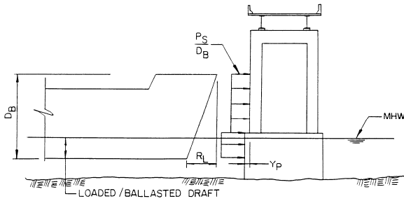
Figure 3.14.14.1-2—Ship Impact Line Load on Pier
