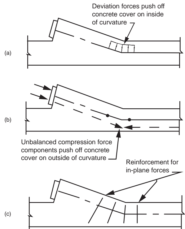
Figure C5.10.4.3.1a-1—In-Plane Forces in a Soffit Blister
