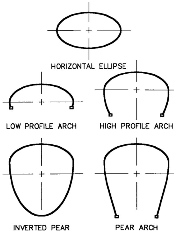
Figure 12.8.1-1—Long-Span Shapes
