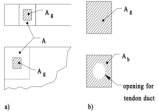
Figure C5.10.9.7.2-1—Area of Supporting Concrete Surface in Eq. 5.10.9.7.2-2
