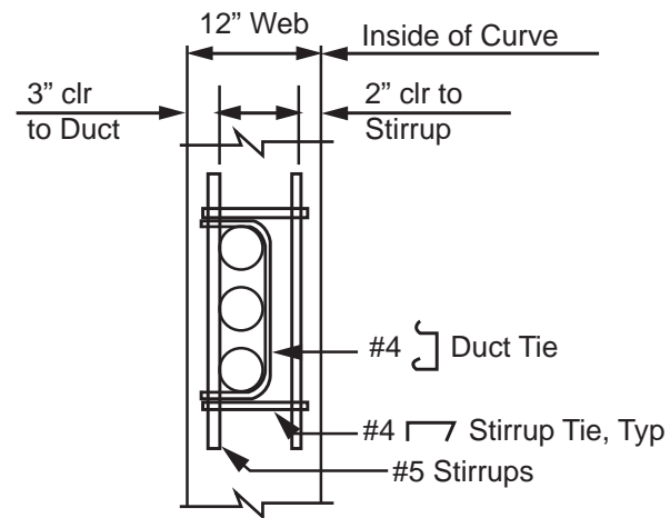
Figure C5.10.4.3.1b-1—Typical Stirrup and Duct Tie Detail
