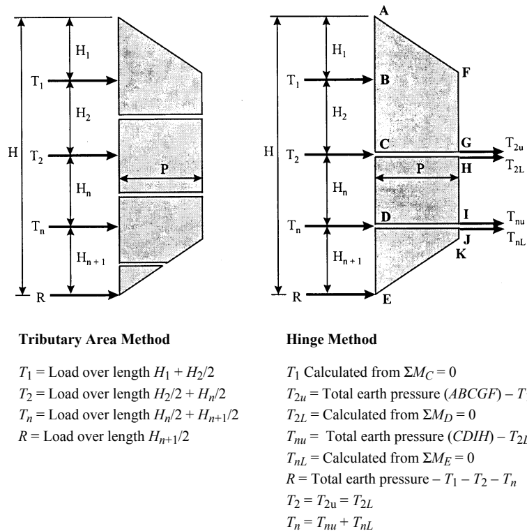
Figure C11.9.5.1-2—Calculation of Anchor Loads for Multilevel Wall after Sabatini et al. (1999)
