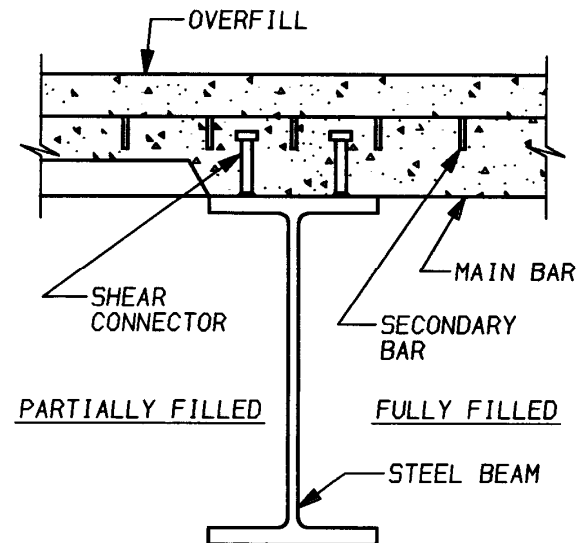
Figure C9.8.2.3.1-1—An Acceptable Shear Connection of Partially and Fully Filled Grid Decks to Beams
