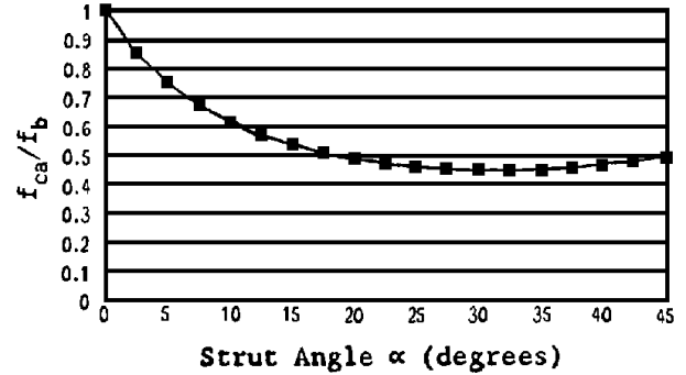
Figure C5.10.9.6.2-1—Local Zone and Strut Interface
