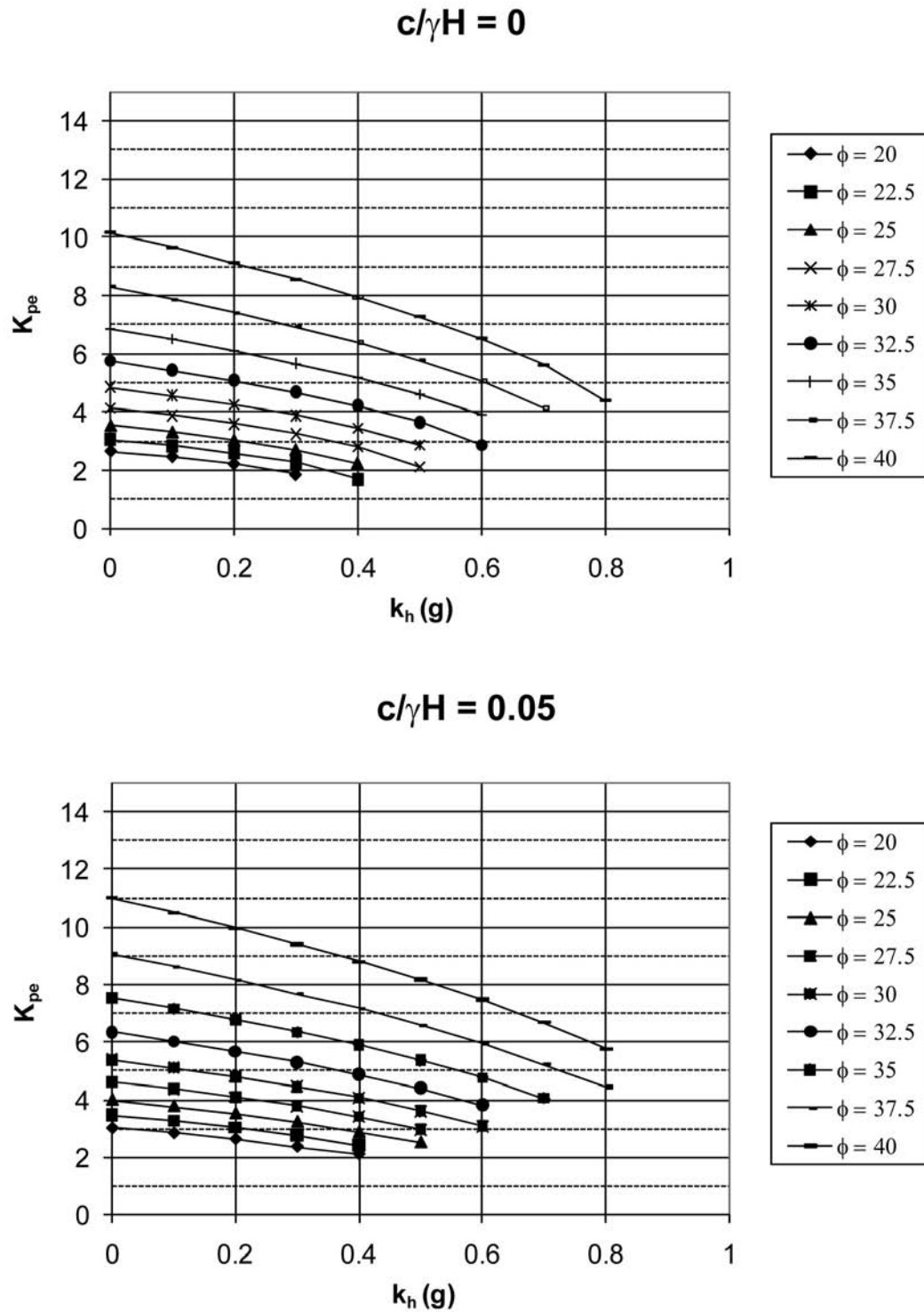
Figure A11.4-2—Seismic Passive Earth Pressure Coefficient Based on Log Spiral Procedure for c/\gamma H = 0 and 0.05 ( c = soil cohesion, \gamma = soil unit weight, and H = height or depth of wall over which the passive resistance acts)
