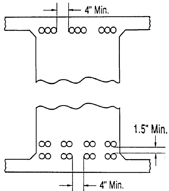
Figure C5.10.3.3.2-1—Examples of Acceptable Arrangements for Ducts Not Curved in the Horizontal Plan
