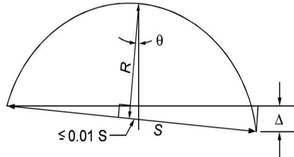
Figure C12.8.4.1-1—Differential Settlement
