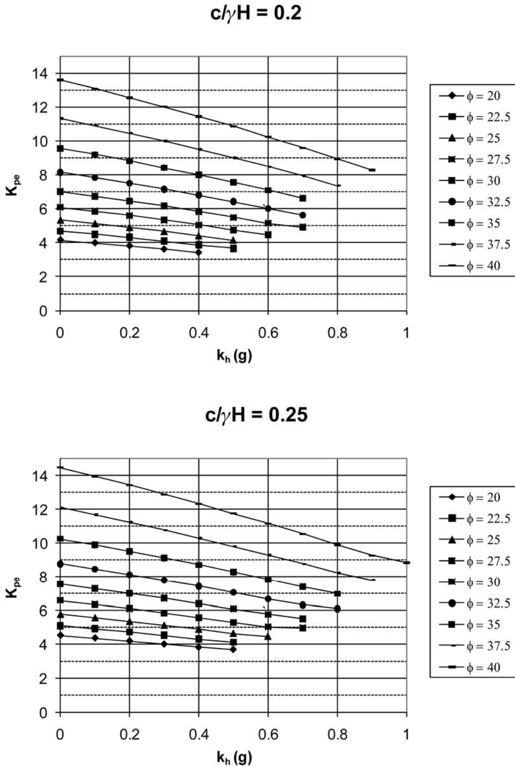
Figure A11.4—Seismic Passive Earth Pressure Coefficient Based on Log Spiral Procedure for c/\gamma H = 0.2 and 0.25 ( c = soil cohesion, \gamma = soil unit weight, and H = retaining wall height or depth of wall over which the passive resistance acts)
