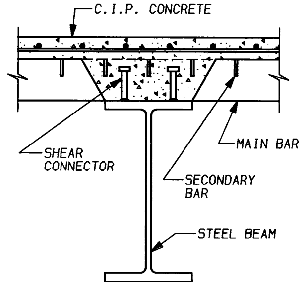
Figure C9.8.2.4.1-1—An Acceptable Shear Connection of Unfilled Grid Decks Composite with Reinforced Concrete Slabs to Beams
