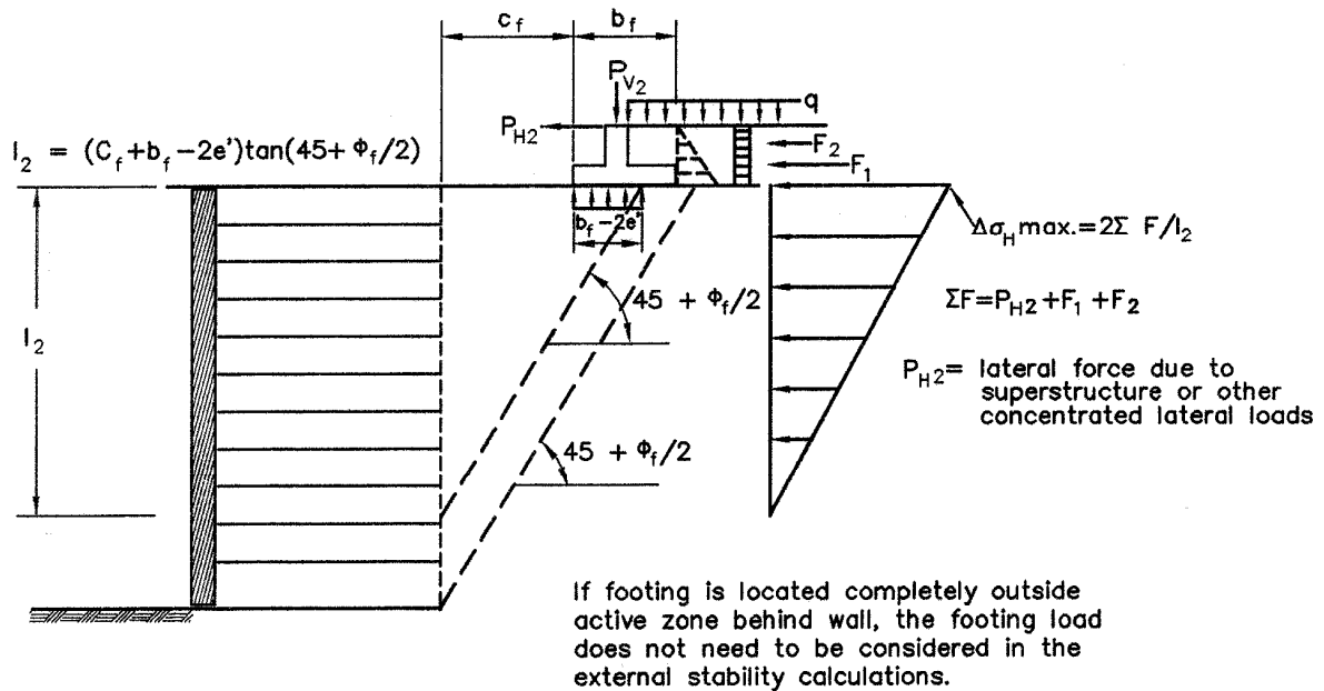
b—Distribution of Stress for External Stability Calculations
