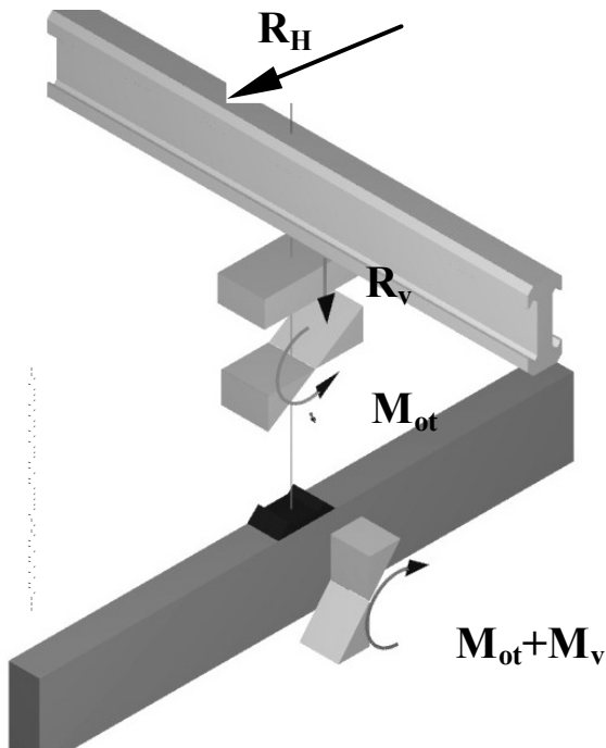
Figure 14.5.6.9.7b-2—Force Effects Associated with Type B Cracking
