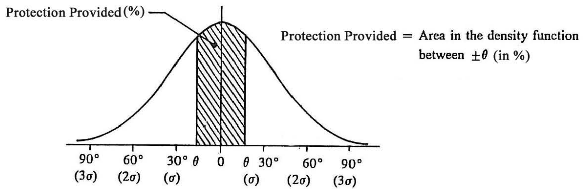
b. Normal Distribution of Vessel Collision Trajectories Around Bridge Pier ( \sigma assumed = 30^\circ ).
