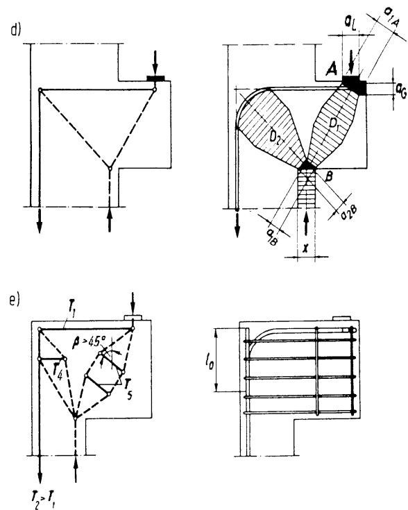
Figure C5.13.2.4.1-1 (continued) —Different Support Conditions Leading to Different Strut-and-Tie Models and Different Reinforcement Arrangements of Corbels and Beam Ledges (Schlaich et al., 1987)
