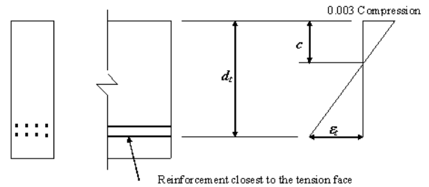
Figure C5.7.2.1-1—Strain Distribution and Net Tensile Strain
