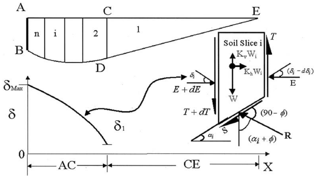
Figure A11.4-1—Limits and Shape Seismic Interslice Force Function (reported in Anderson et al., 2008)
