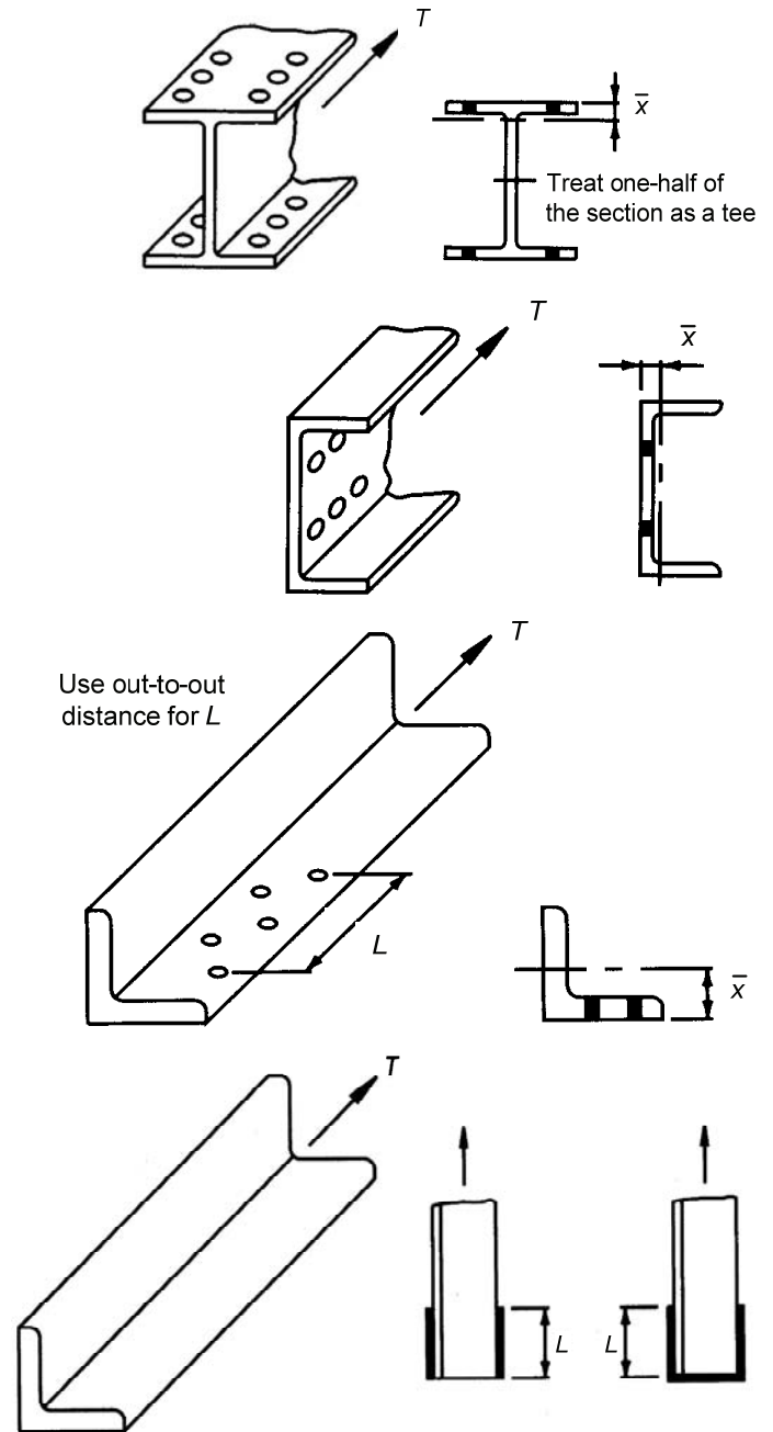
Figure C6.8.2.2-1—Determination of \bar{x} or L in the Calculation of the Shear Lag Reduction Factor, U
