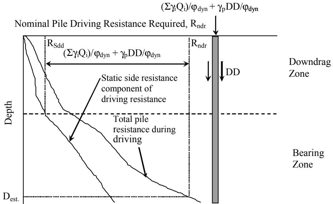
Figure C10.7.3.7-1—Design of Pile Foundations for Downtag
