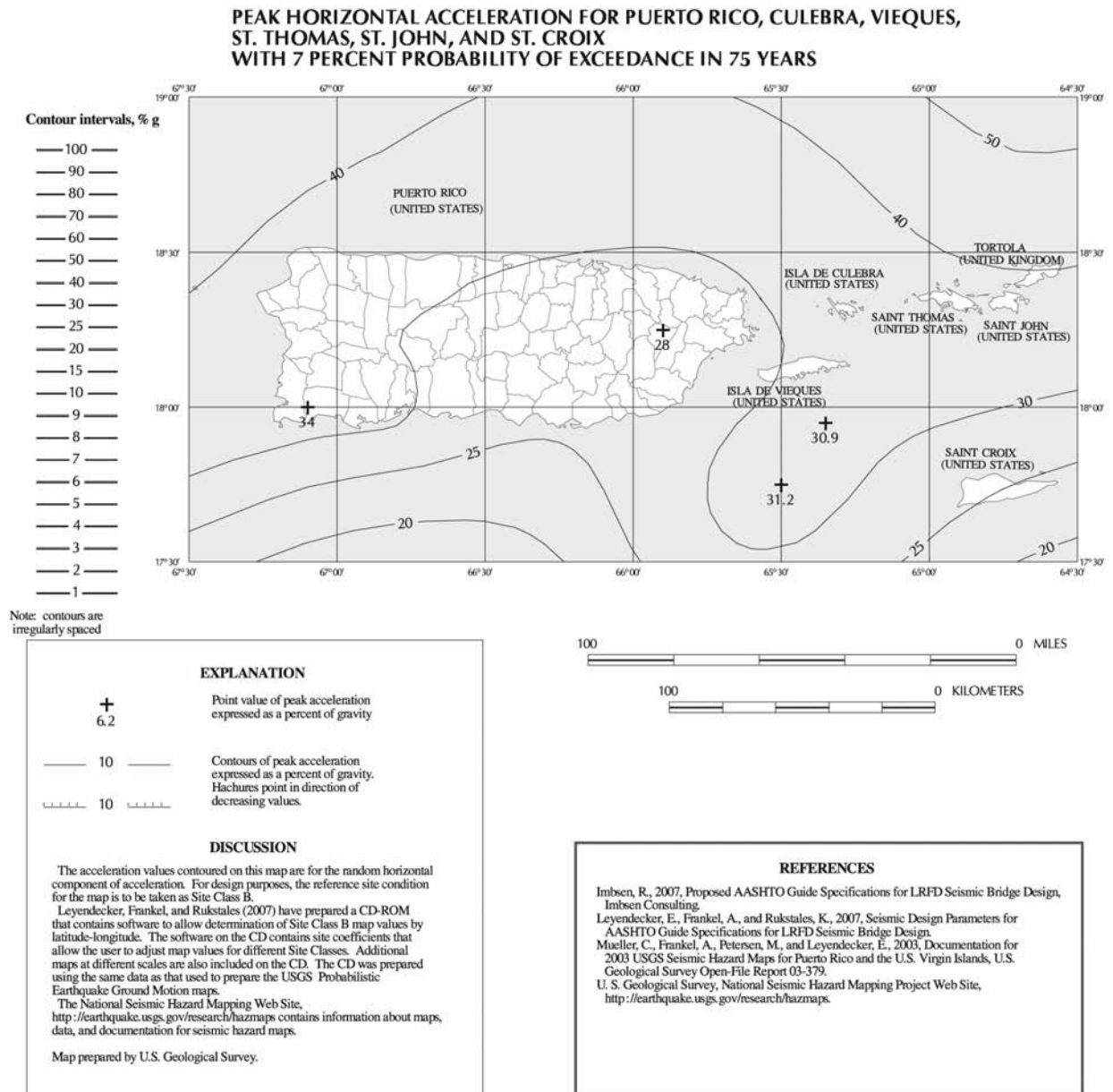
Figure 3.10.2.1-20—Horizontal Peak Ground Acceleration Coefficient for Puerto Rico, Culebra, Vieques, St. Thomas, St. John, and St. Croix (PGA) with Seven Percent Probability of Exceedance in 75 yr (Approx. 1000-yr Return Period)
