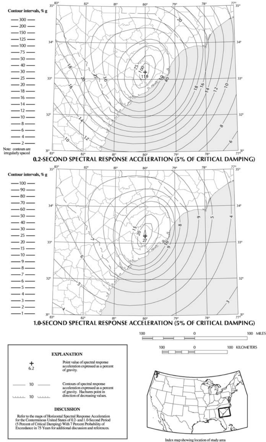
Figure 3.10.2.1-14—Horizontal Response Spectral Acceleration Coefficients for Region 4 at Periods of 0.2 s ( S_0 ) and 1.0 s ( S_1 ) with Seven Percent Probability of Exceedance in 75 yr (Approx. 1000-yr Return Period) and Five Percent Critical Damping
