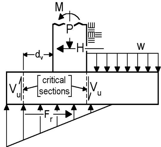
Figure C5.13.3.6.1-1—Example of Critical Section for Shear in Footings
