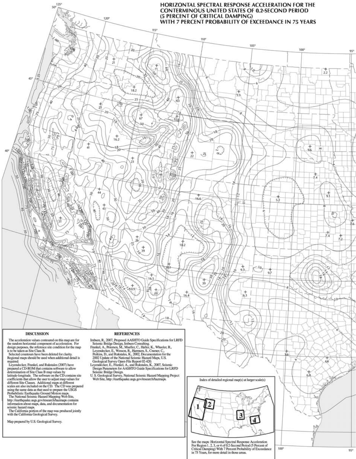
Figure 3.10.2.1-2—Horizontal Response Spectral Acceleration Coefficient for the Conterminous United States at Period of 0.2 s ( S_S ) with Seven Percent Probability of Exceedance in 75 yr (Approx. 1000-yr Return Period) and Five Percent Critical Damping
