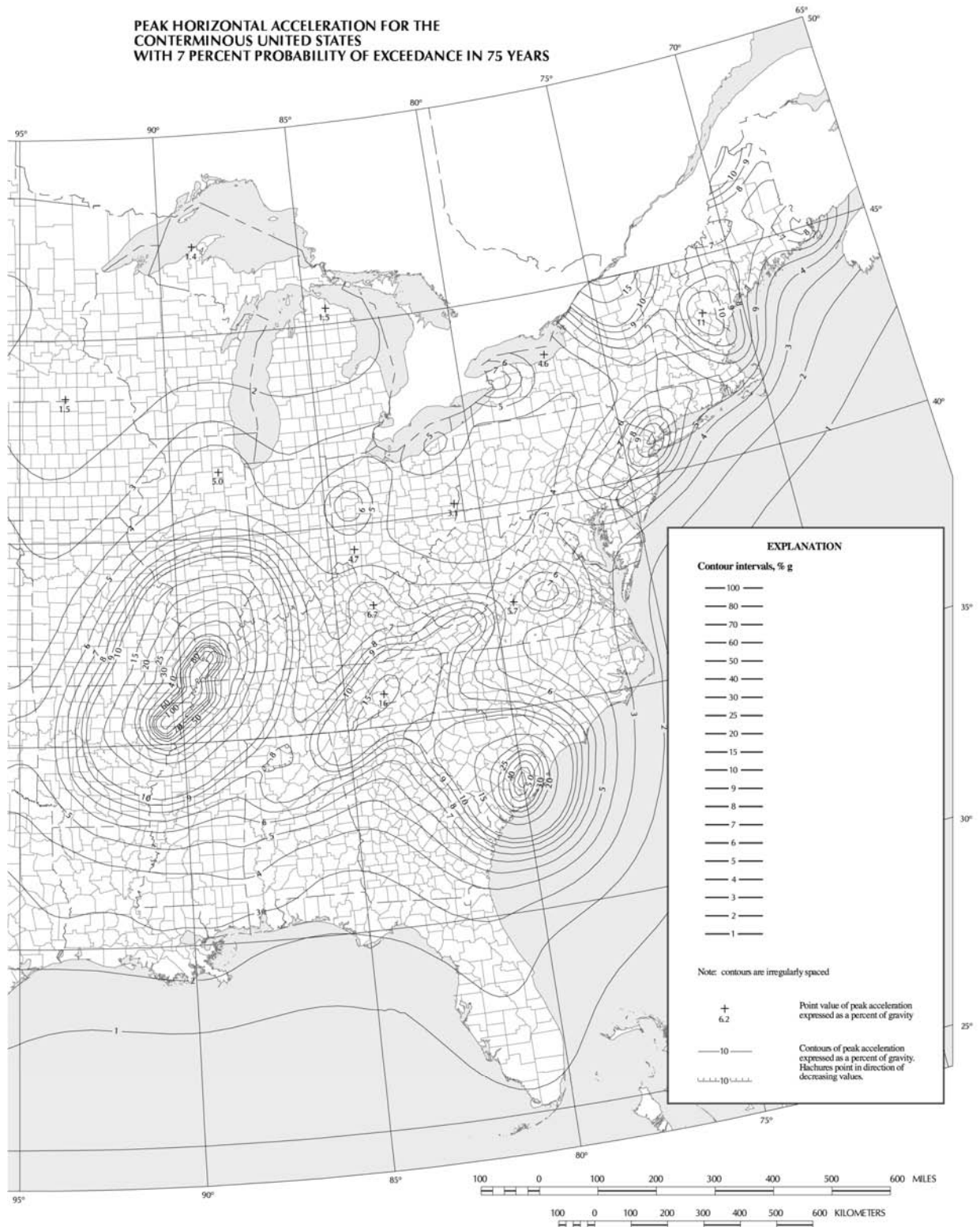
Figure 3.10.2.1-1 (continued)—Horizontal Peak Ground Acceleration Coefficient for the Conterminous United States (PGA) with Seven Percent Probability of Exceedance in 75 yr (Approx. 1000-yr Return Period)
