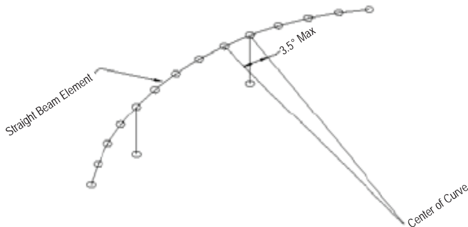
Figure 4.6.1.2.3-2—Three-Dimensional Spine Model of Curved Concrete Box Girder Bridge
