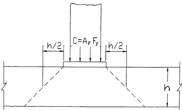
Figure A13.4.3.2-1—Punching Shear Failure Mode
