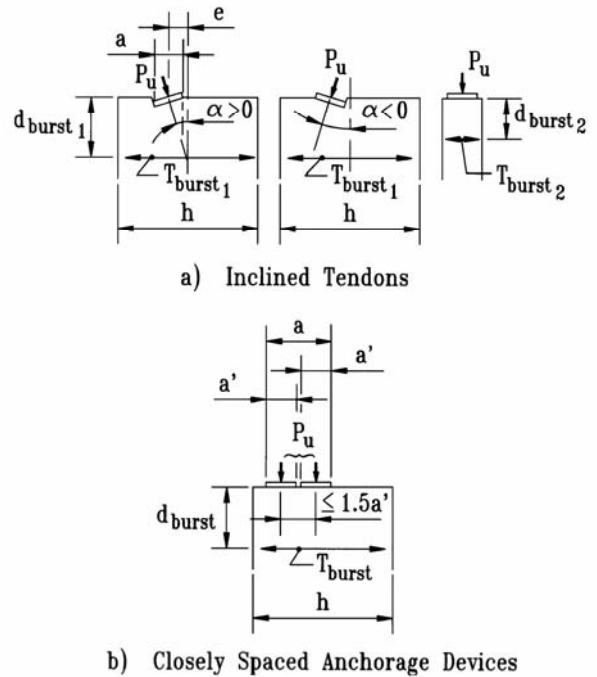
Figure C5.10.9.6.3-1—Notation for Eqs. 5.10.9.6.3-1 and 5.10.9.6.3-2
