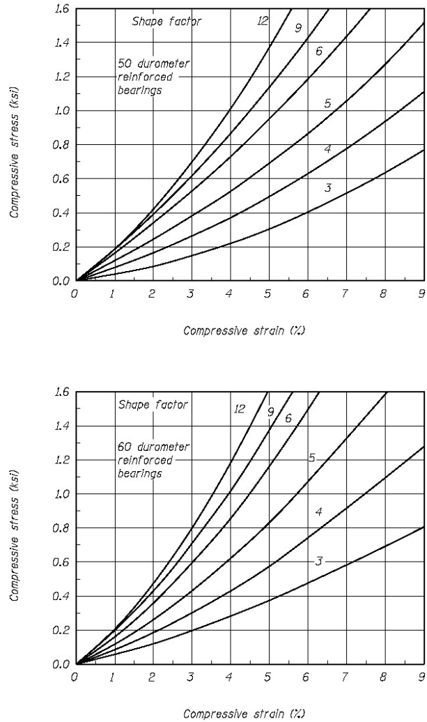
Figure C14.7.6.3.3-1—Stress-Strain Curves
