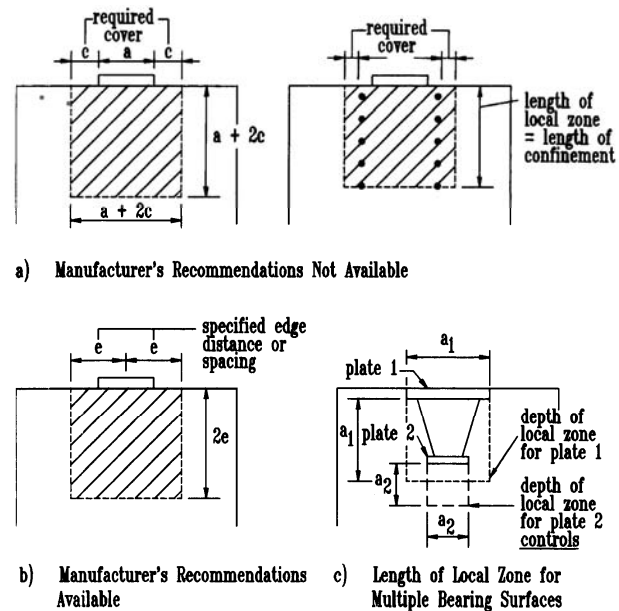
Figure C5.10.9.7.1-1—Geometry of the Local Zone
