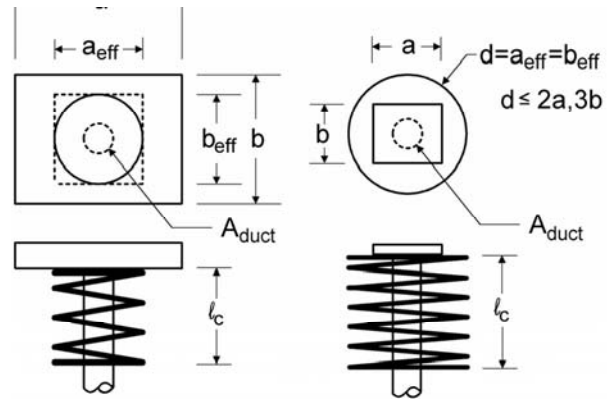
Figure C5.10.9.6.2-3—Effective Bearing Area
