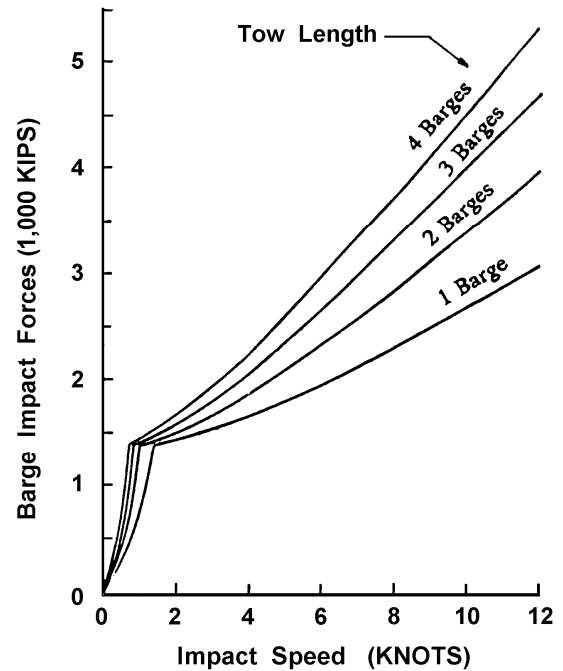
Figure C3.14.11-2—Typical Hopper Barge Impact Forces
