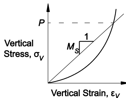
Figure C12.12.3.5-1—Schematic One-Dimensional Stress-Strain Curve of Soil Backfill
