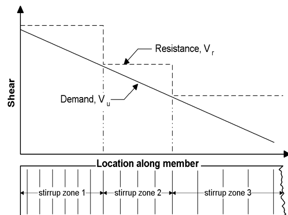
Figure C5.8.3.2-1—Traditional Shear Design
