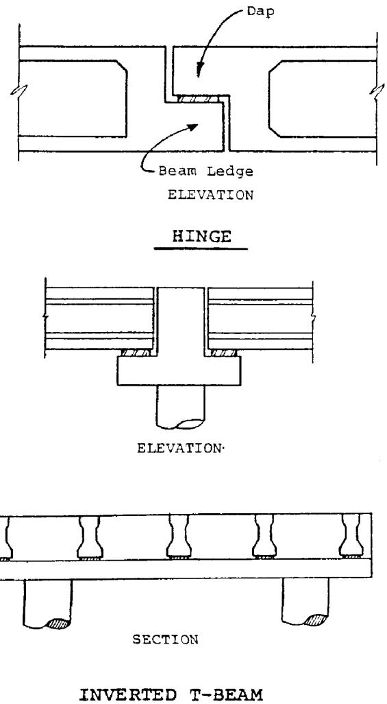
Figure C5.13.2.5.1-1—Examples of Beam Ledges
