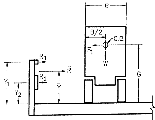
Figure CA13.2-1—Traffic Railing
