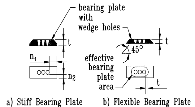
Figure C5.10.9.7.2-3—Effective Bearing Plate Area for Anchorage Device without Separate Wedge Plate
