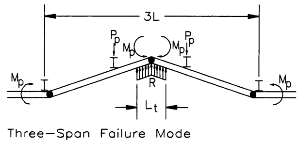
Figure CA13.3.2-1—Possible Failure Modes for Post-and-Beam Railings
