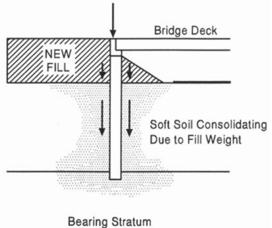
Figure C3.11.8-1—Common Downdrag Situation Due to Fill Weight (Hannigan, et al., 2005)
