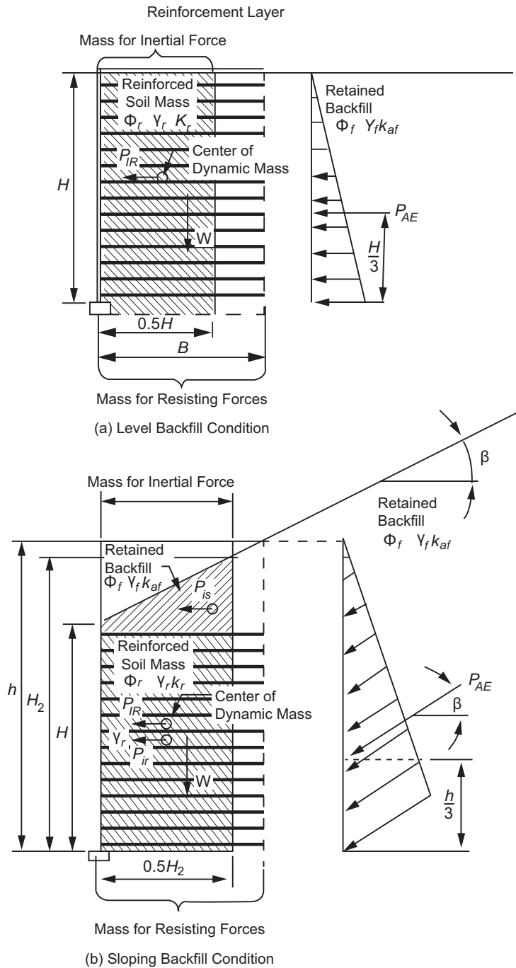
Figure 11.10.7.1-1—Seismic External Stability of an MSE Wall
