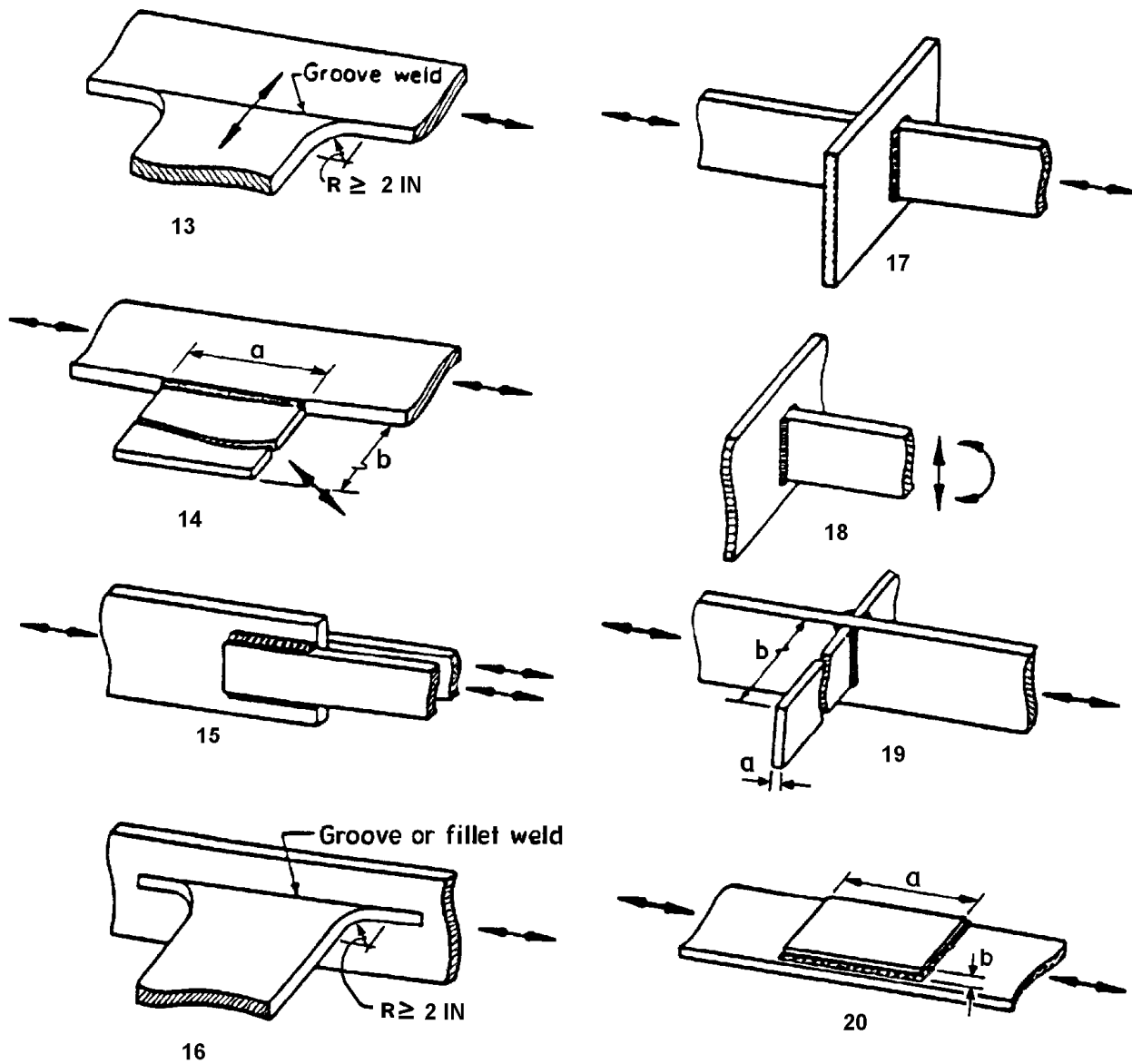
Figure 7.6.1.2.3-1— Illustrative Examples (continued)
