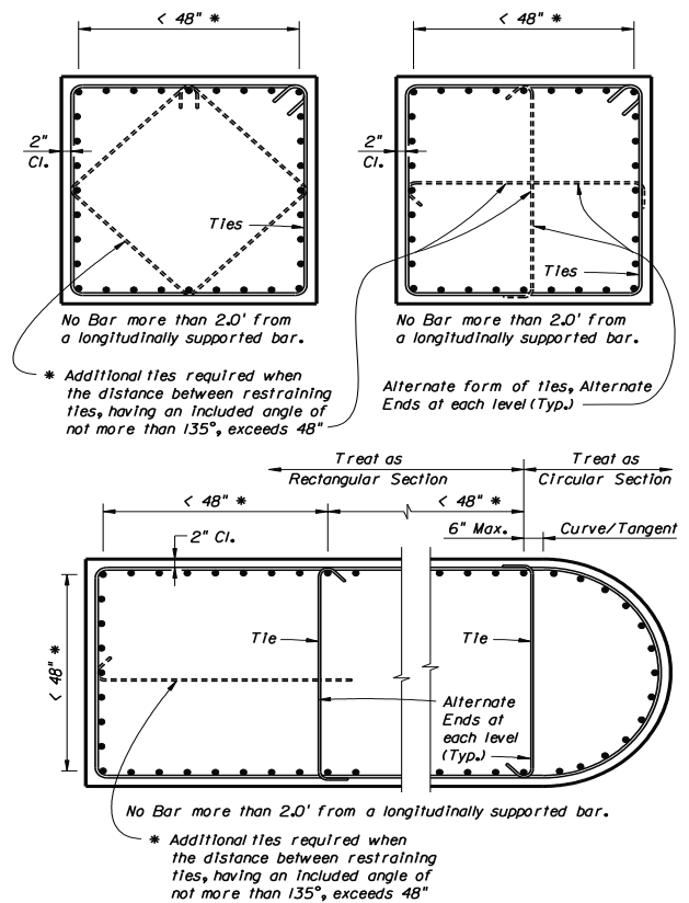
Figure C5.10.6.3-1—Acceptable Tie Arrangements
