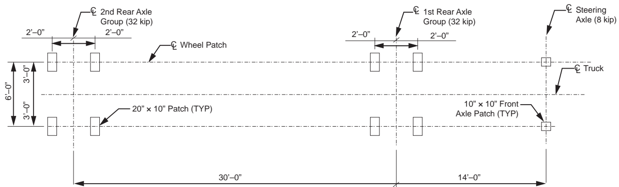
Figure 3.6.1.4.1-1—Refined Design Truck Footprint for Fatigue Design
