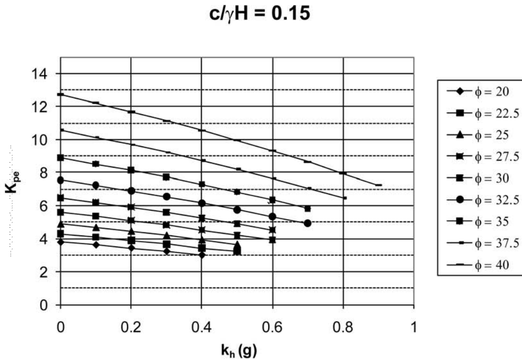
Figure A11.4-3—Seismic Passive Earth Pressure Coefficient Based on Log Spiral Procedure for c/\gamma H = 0.1 and 0.15 ( c = soil cohesion, \gamma = soil unit weight, and H = retaining wall height or depth of wall over which the passive resistance acts)
