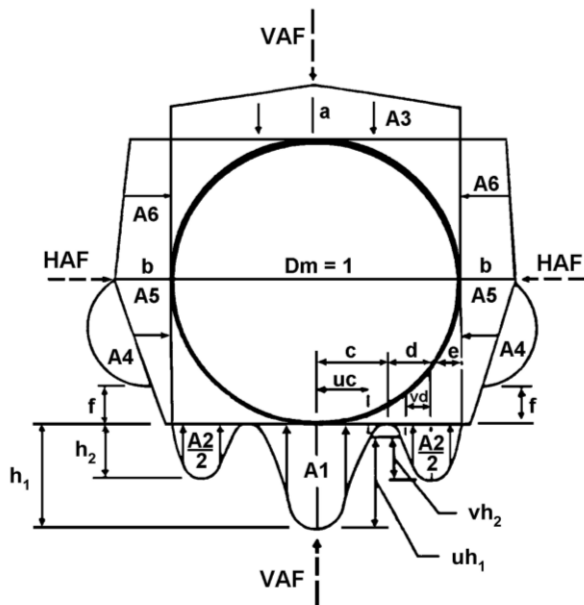
Figure 12.10.2.1-1—Heger Pressure Distribution and Arching Factors
