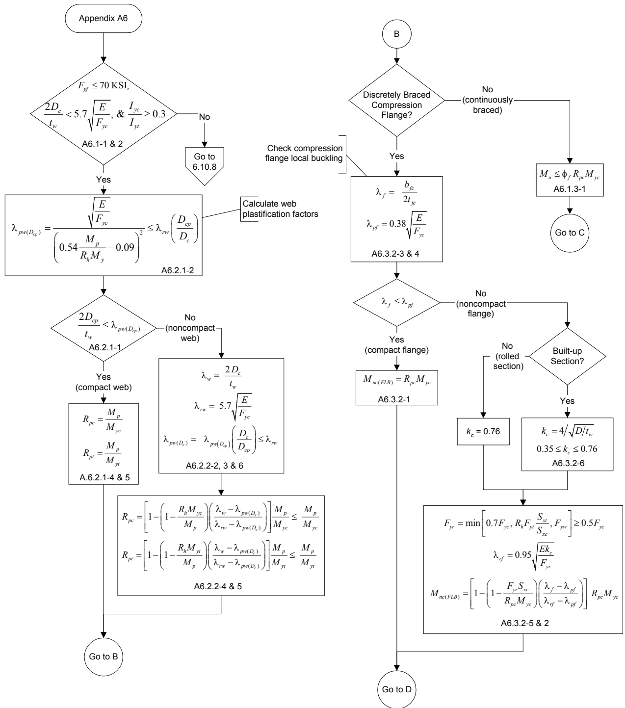
Figure C6.4.7-1—Flowchart for Appendix A6—Flexural Resistance of Straight Composite I-Sections in Negative Flexure and Straight Noncomposite I-Sections with Compact or Noncompact Webs
