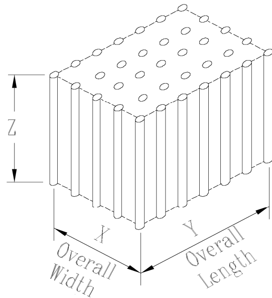
Figure C10.7.3.9-1—Pile Group Acting as a Block Foundation
