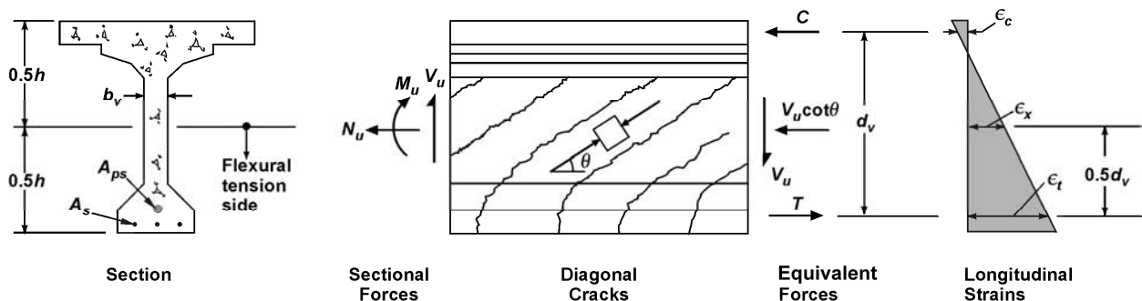
Figure B5.2-1—Illustration of Shear Parameters for Section Containing at Least the Minimum Amount of Transverse Reinforcement, V_p = 0
