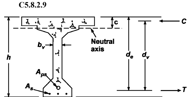
Figure C5.8.2.9-1—Illustration of the Terms b_v and d_v
