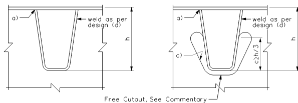
a) Intersections of closed ribs with floorbeams.
