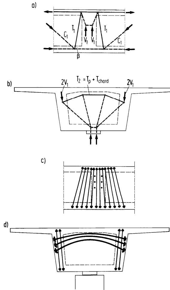
Figure C5.13.2.2-1—Diaphragm of a Box Girder Bridge: (a) Disturbed Regions and Model of the Web near the Diaphragm; (b) Diaphragm and Model; (c) and (d) Prestressing of the Web and the Diaphragm (Schlaich et al., 1987)
