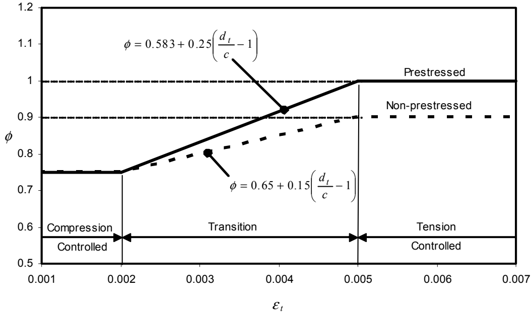
Figure C5.5.4.2.1-1—Variation of \phi with Net Tensile Strain \epsilon_t and d_t/c for Grade 60 Reinforcement and for Prestressing Steel
