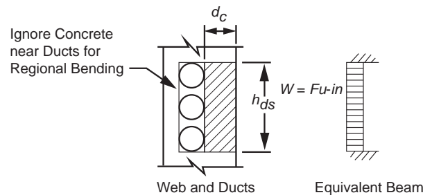
Figure C5.10.4.3.1c-1—Hypothetical Unreinforced Concrete Cover Beam
