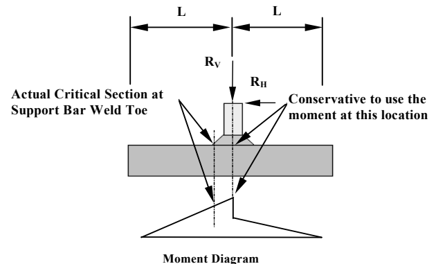
Figure C14.5.6.9.7b-1—Typical Moment Diagram for a Support Bar
