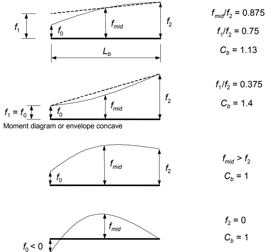
Figure C6.4.10-1—Moment Gradient Modifier, C_b (Sample Cases)
