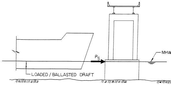
Figure 3.14.14.1-1—Ship Impact Concentrated Force on Pier
