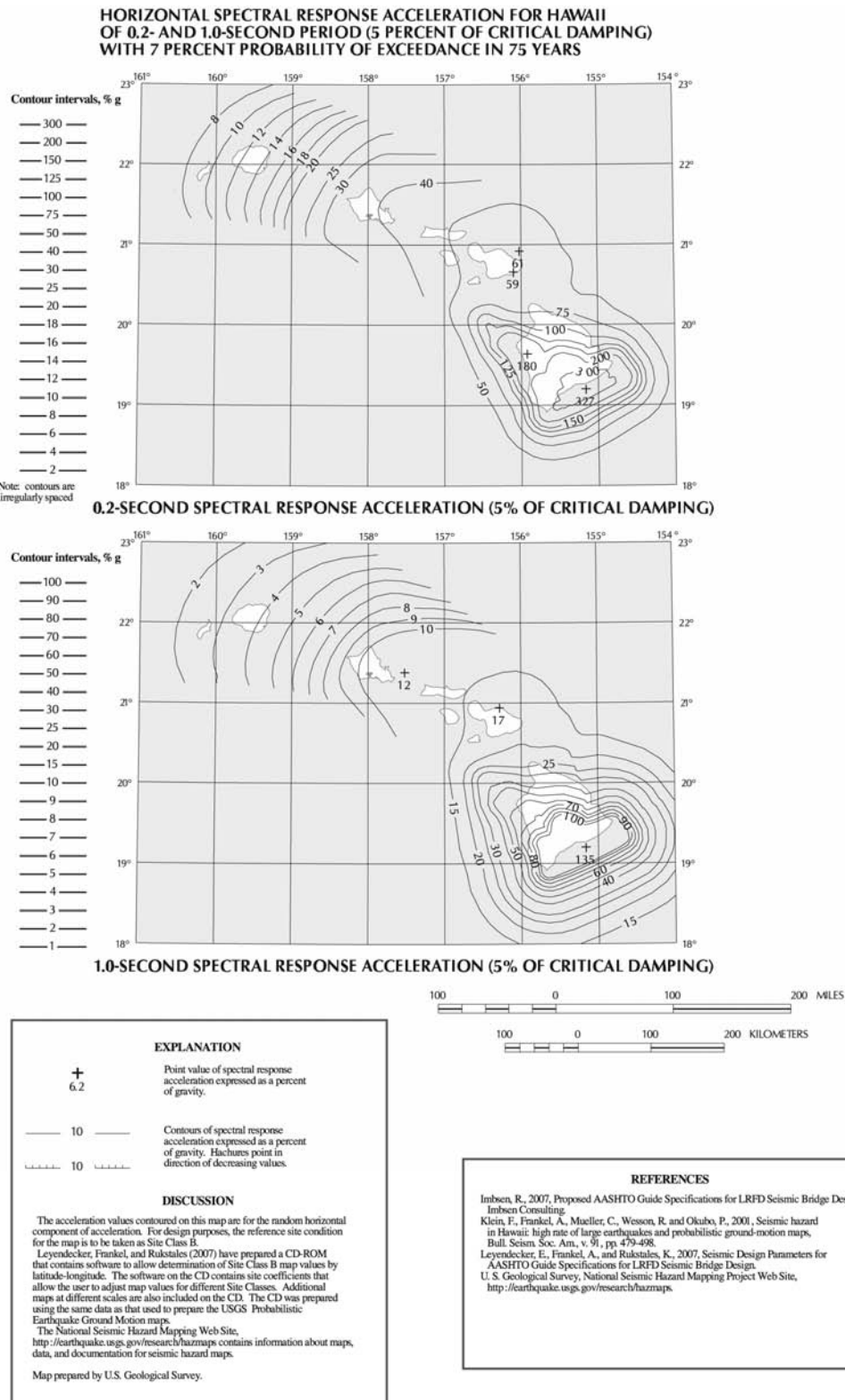
Figure 3.10.2.1-16—Horizontal Response Spectral Acceleration Coefficients for Hawaii at Periods of 0.2 s ( S_0 ) and 1.0 s ( S_1 ) with Seven Percent Probability of Exceedance in 75 yr (Approx. 1000-yr Return Period) and Five Percent Critical Damping
