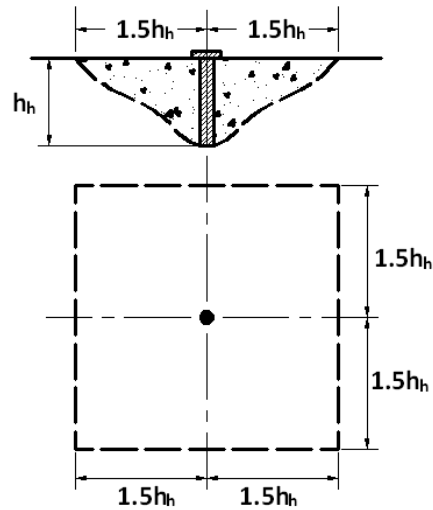
Figure C6.16.4.3-1—Calculation of A_{nco}
