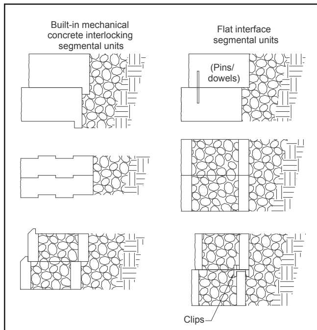
Figure 2—Shear Connectors for SRWs
