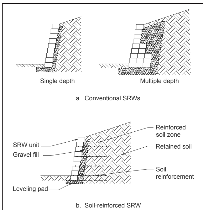
Figure 1—Segmental Retaining Wall Systems
